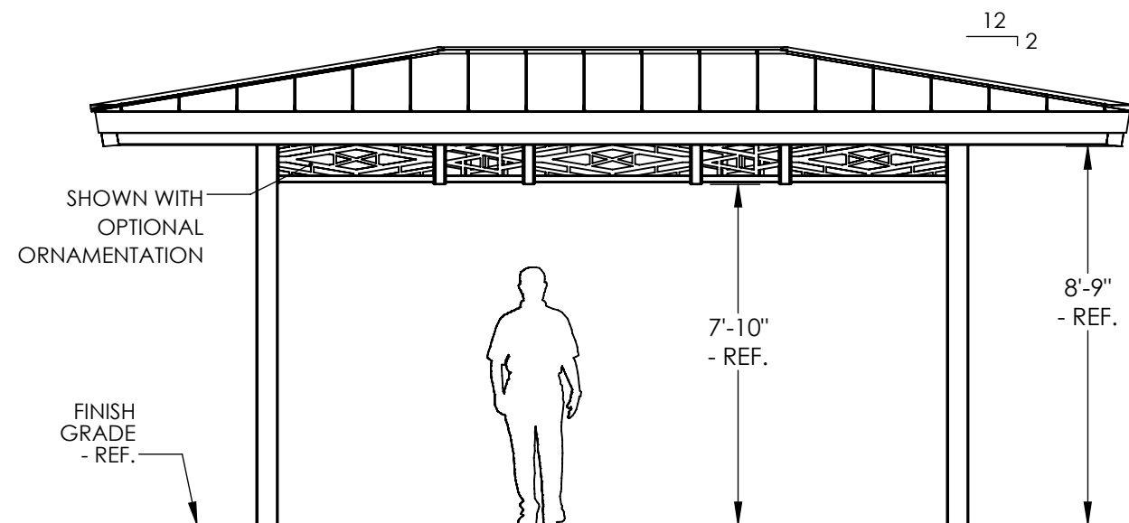
FRONT VIEW
