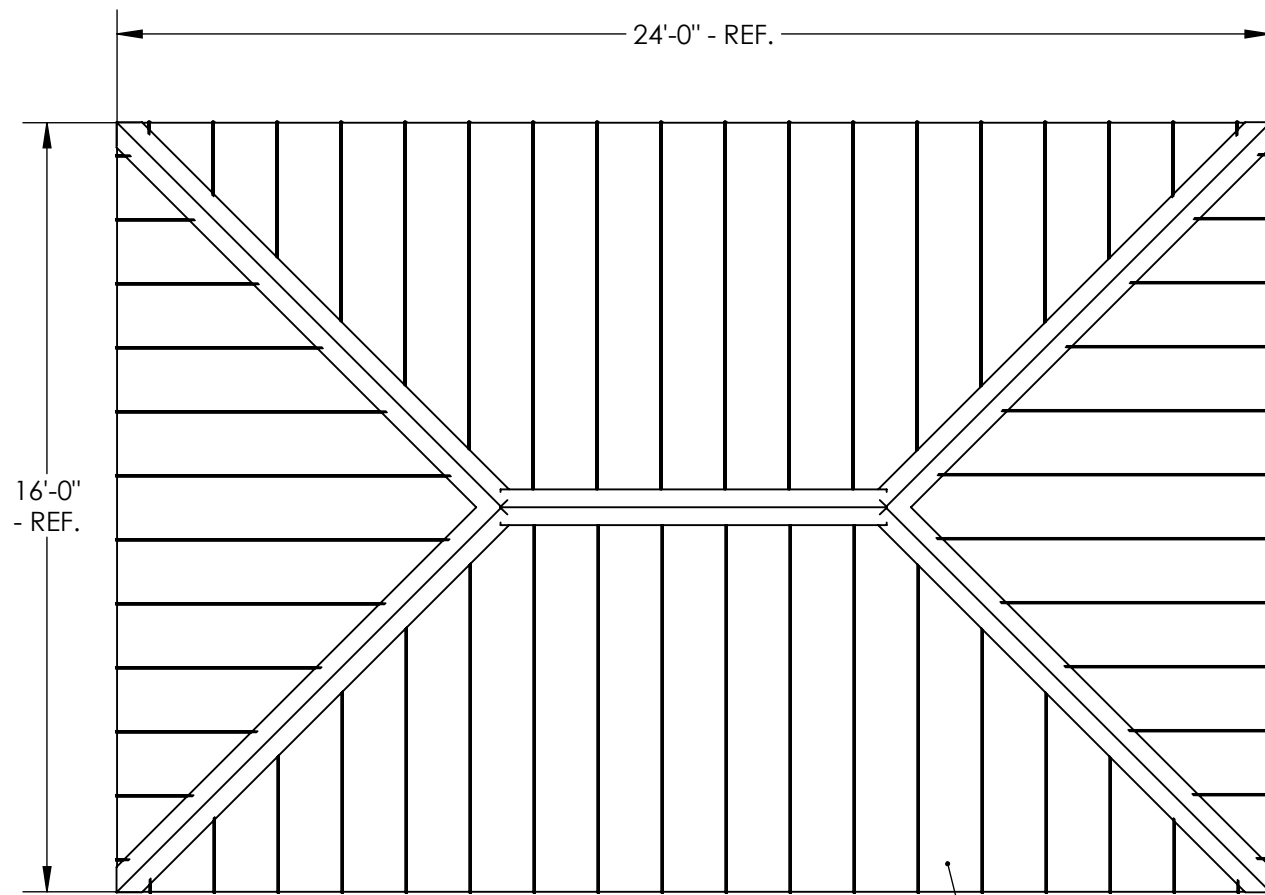
TOP VIEW
