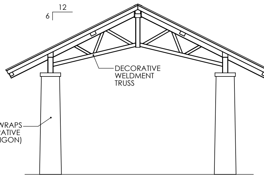
FRONT ELEVATION
